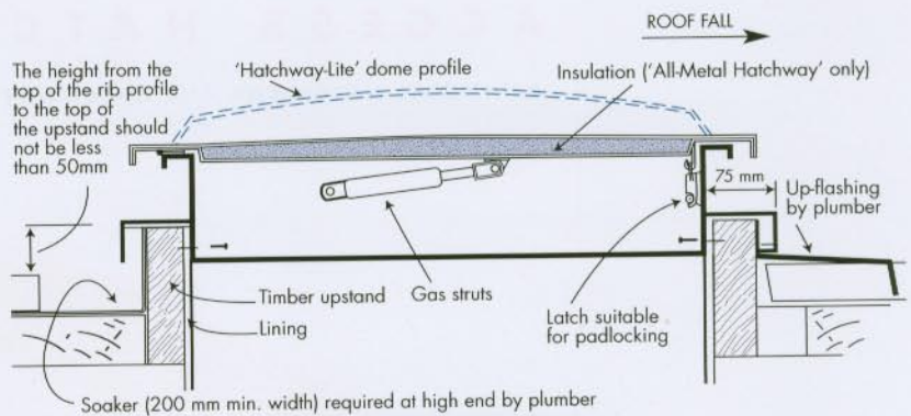
Upstand requirements for correct fitting
